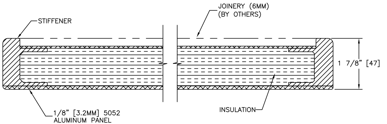
05 WOOD INLAY DOOR PANEL PCM-----05
