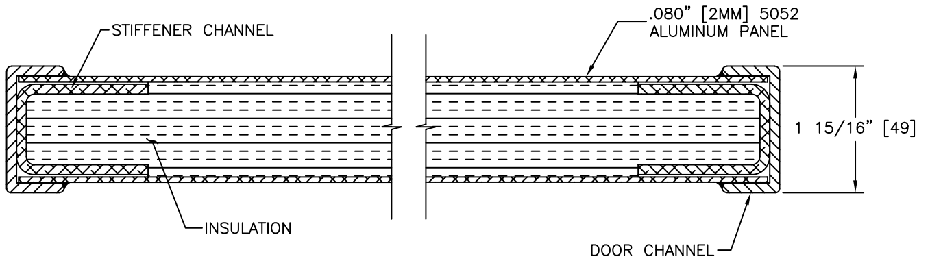
01 CHANNEL DOOR PANEL PCM-----01
