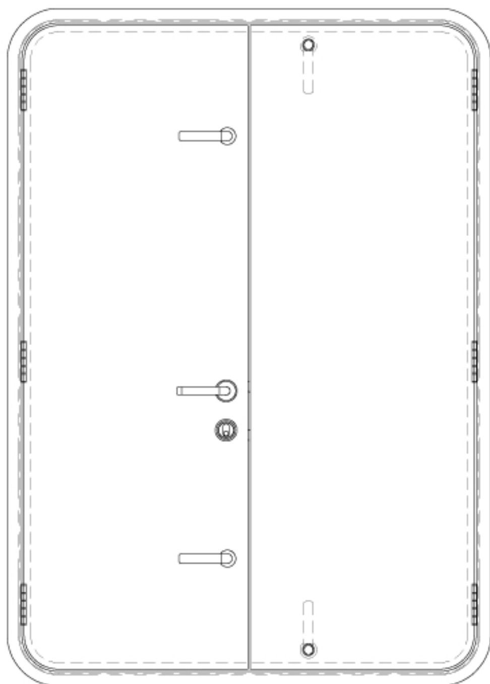
EXTERIOR ELEVATION
